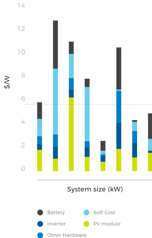
Installed costs of microgrids by region in $/kW, off-grid (2015)
