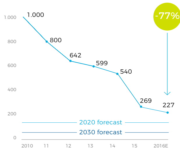
Average battery pack price $ per kWh
